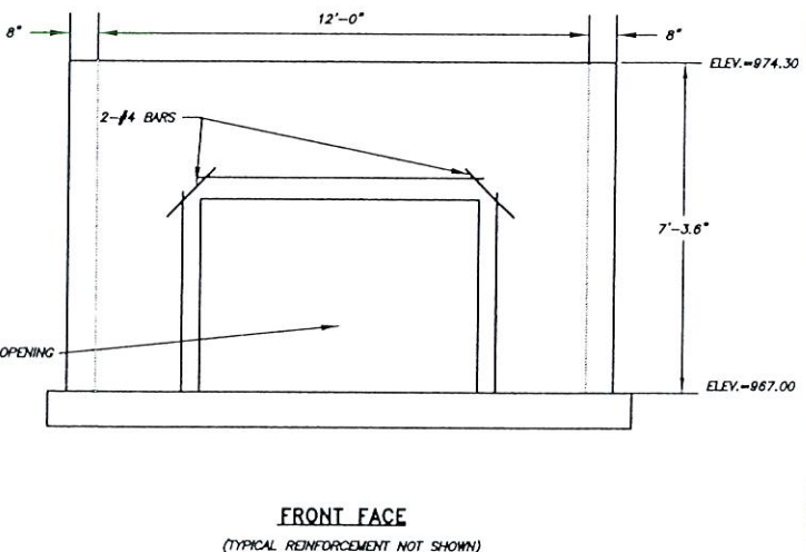
BASIN #2 OUTLET STRUCTURE N.T.S.
