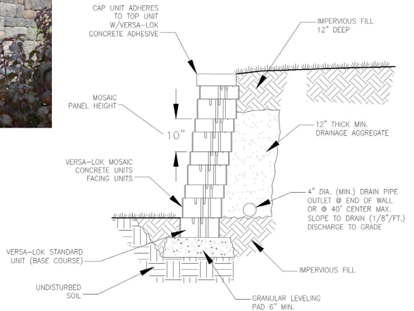
TYPICAL SECTION—UNREINFORCED RETAINING WALL MOSAIC SCALE: NONE
