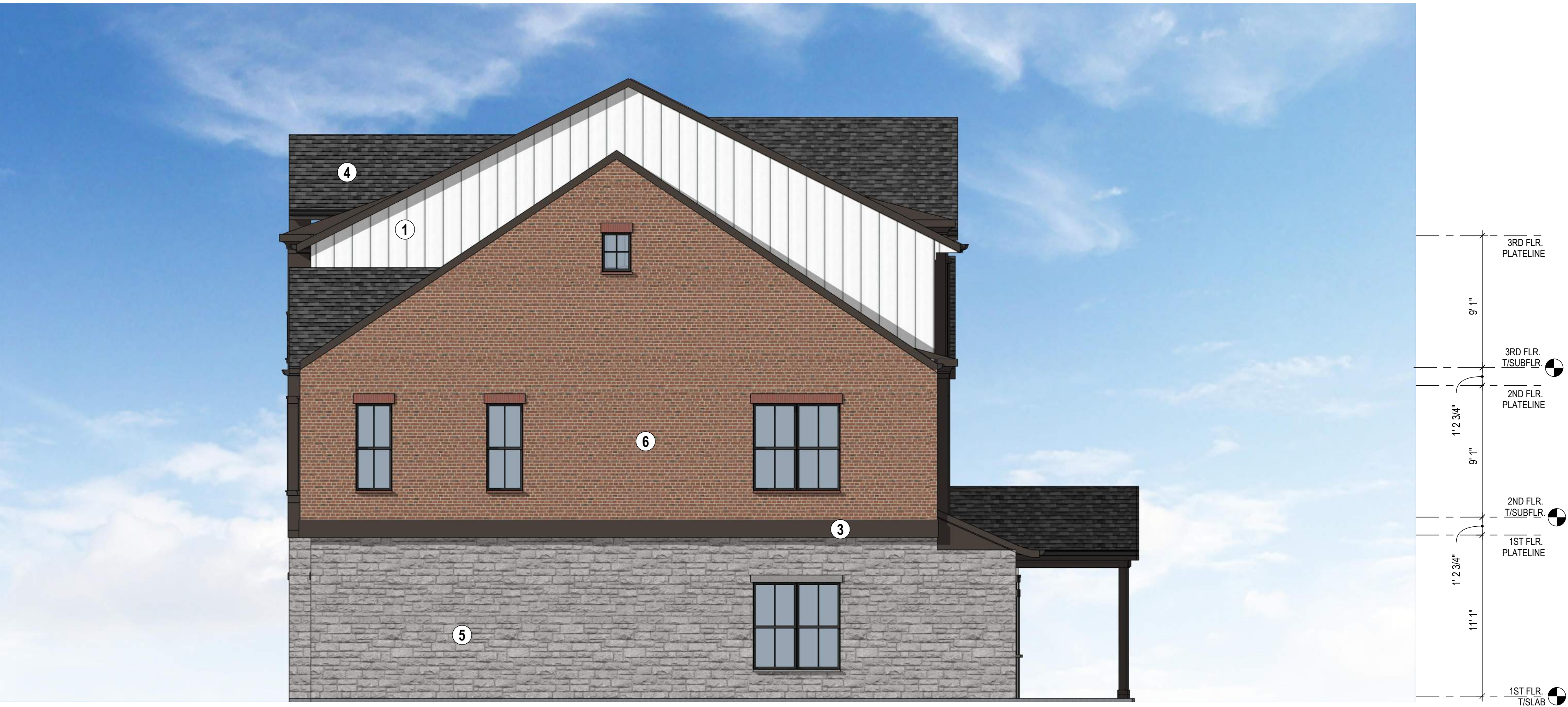
1 LEFT ELEVATION Scale: 3/16" = 1'-0"
