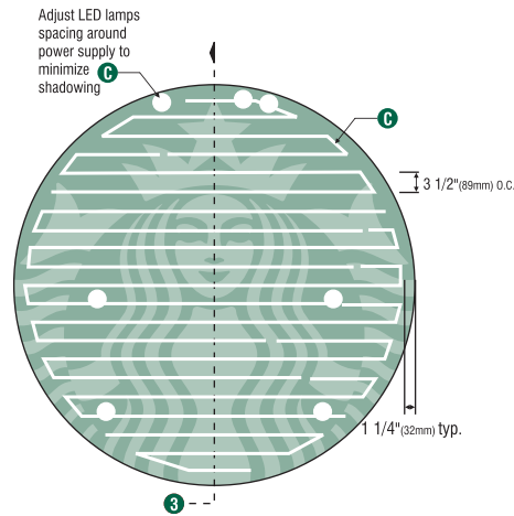
2 LED Detail
