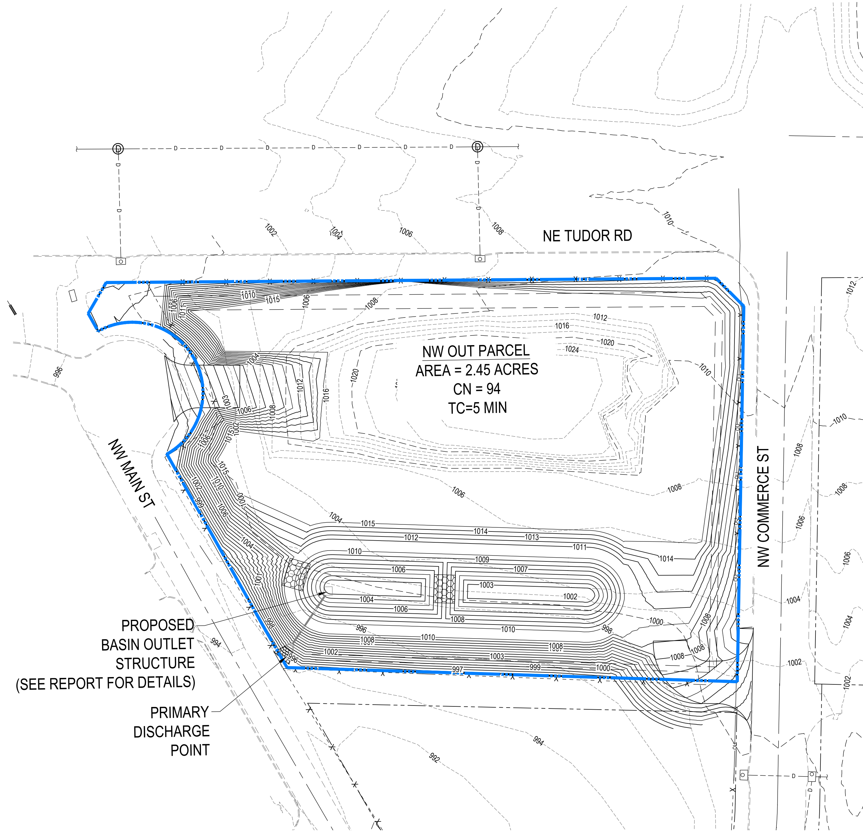
2 NW OUTPARCEL POST DRAINAGE BASINS 1"=40'
