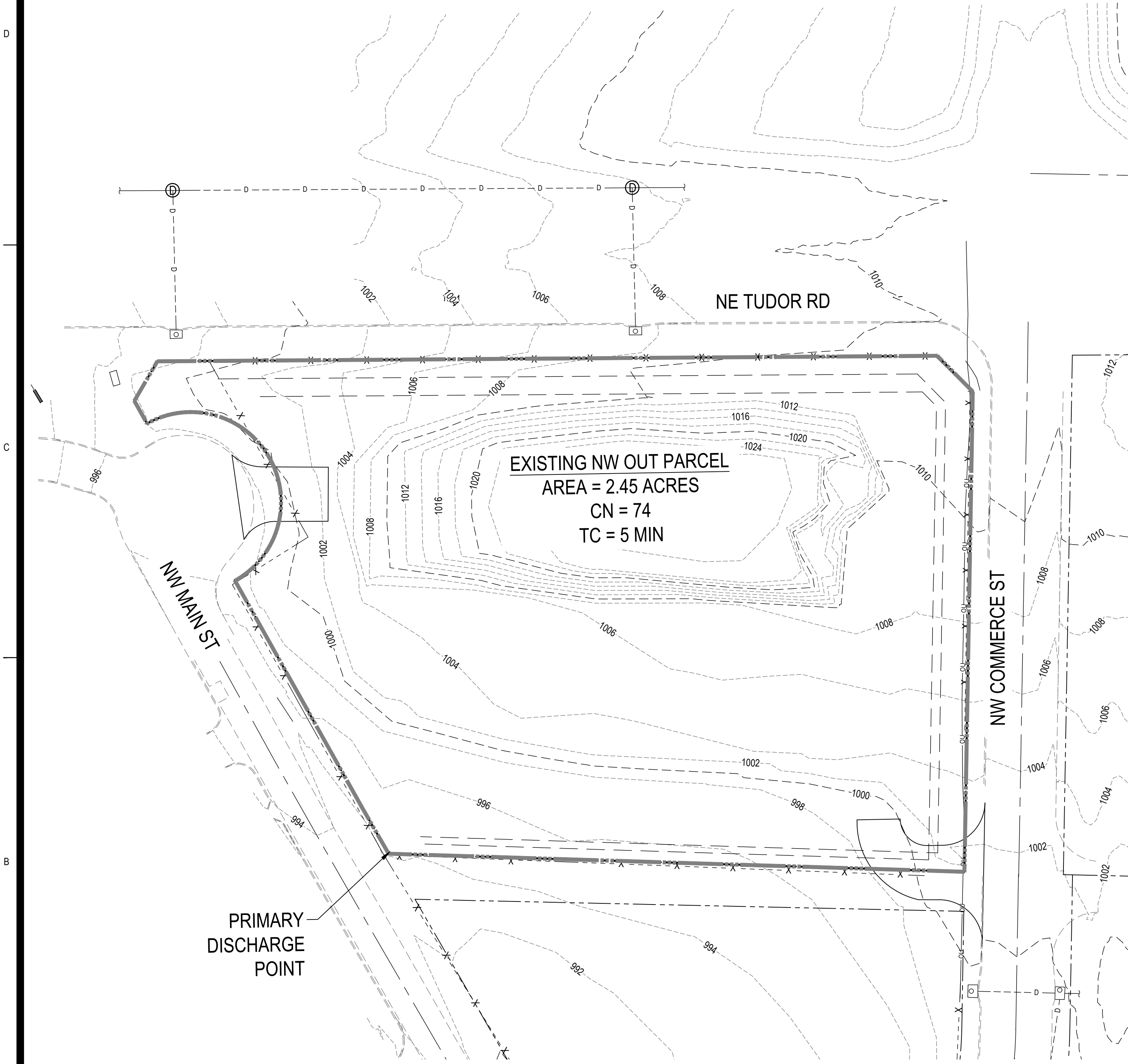
1 NW OUTPARCEL PRE DRAINAGE BASINS 1"=40'
