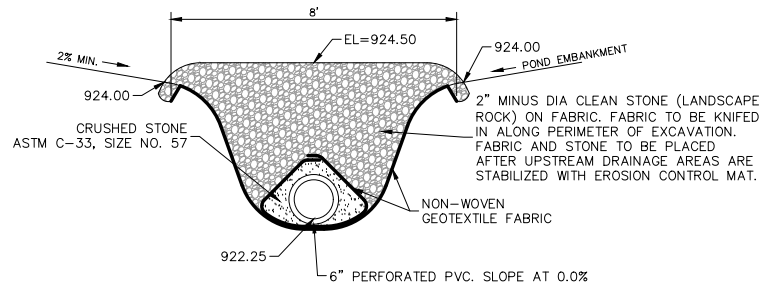
UNDERDRAIN SECTION: A
