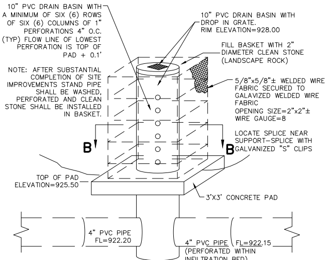
OUTLET STRUCTURE J1 DETAIL NOT TO SCALE
