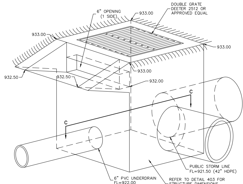
POND OUTLET STRUCTURE PB2 DETAIL
