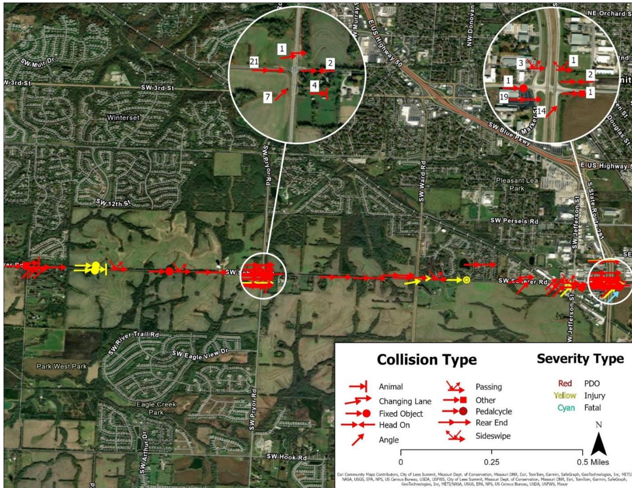
Figure 6 – Existing Corridor Collision Diagram
