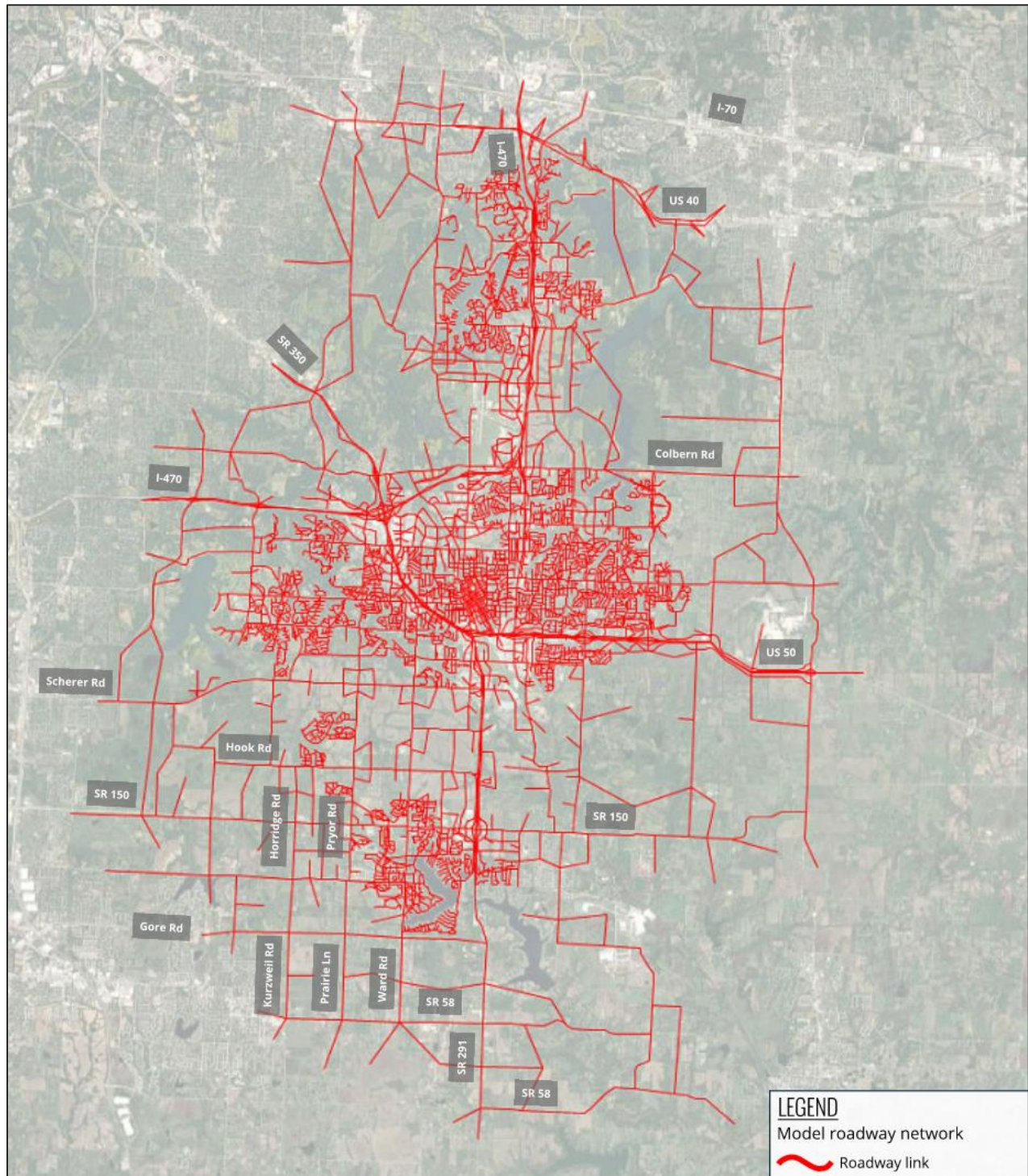
Figure 10 – Model Roadway Network
