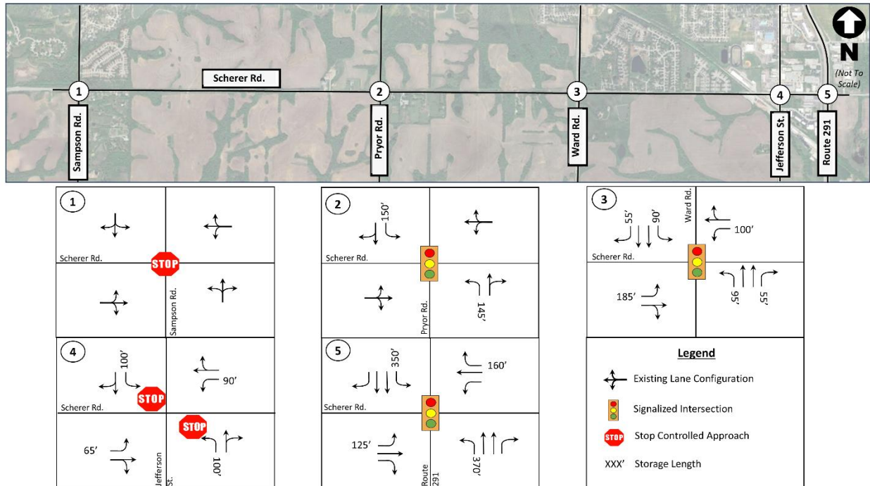
Figure 4 – Existing Intersection Lane Configuration
