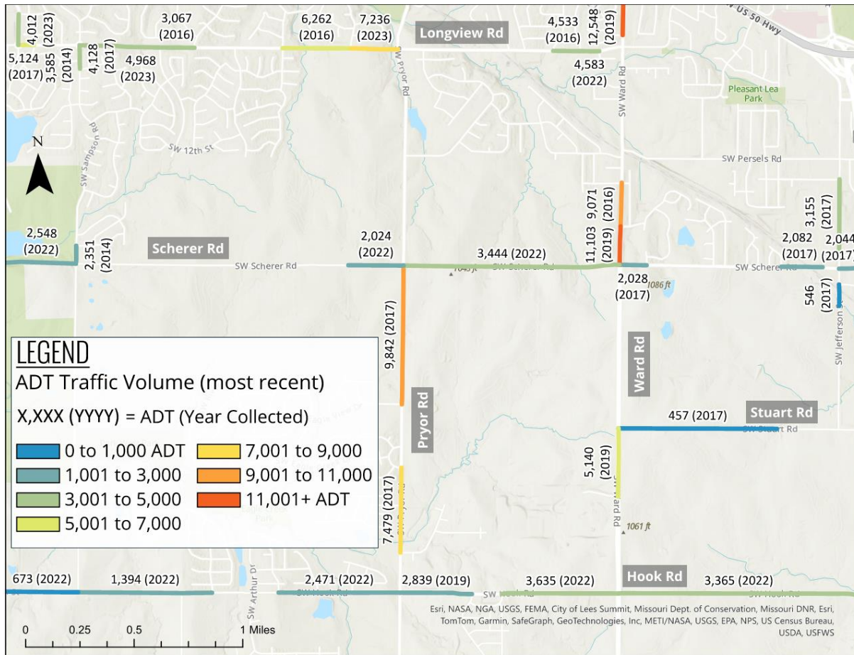
Figure 5 – Existing ADT
