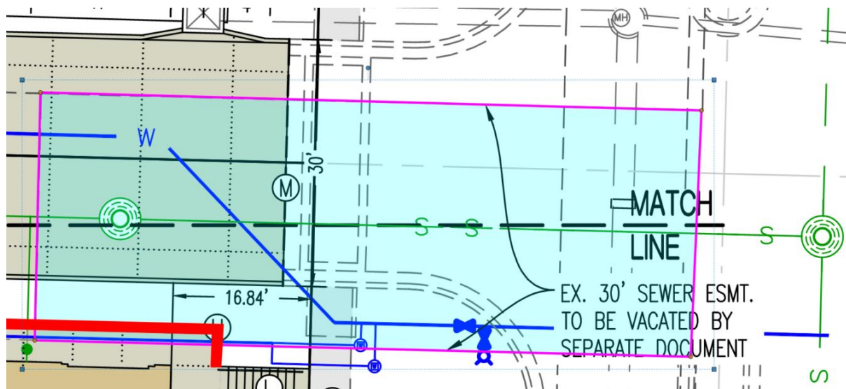
Figure 1 – Easement to be vacated depicted in teal w/ magenta outline. Retaining wall depicted in red.
