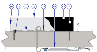
"TOTAL WINE & SPIRITS" PROFILE NOT TO SCALE
