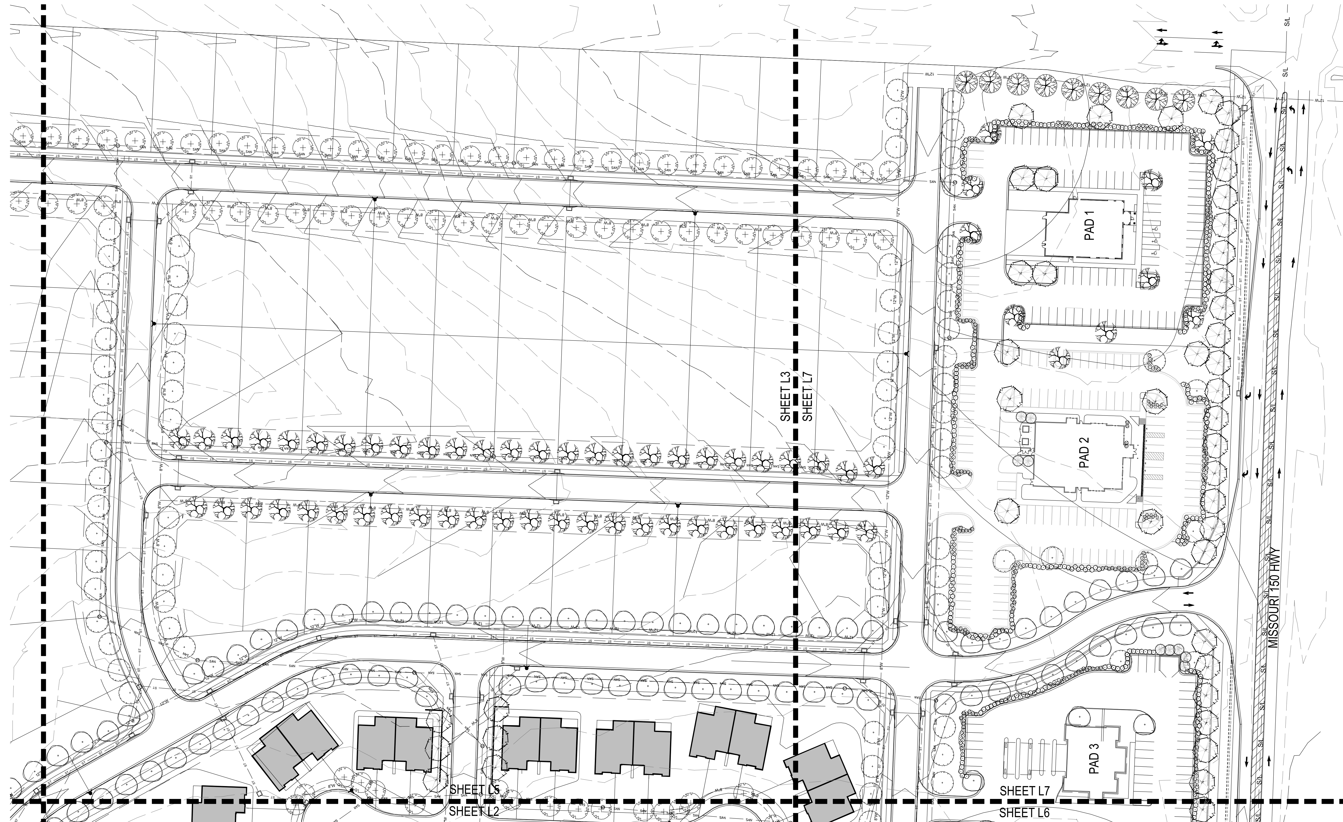
1 LANDSCAPE PLAN ENLARGEMENT SCALE: 1"=50'-0"
