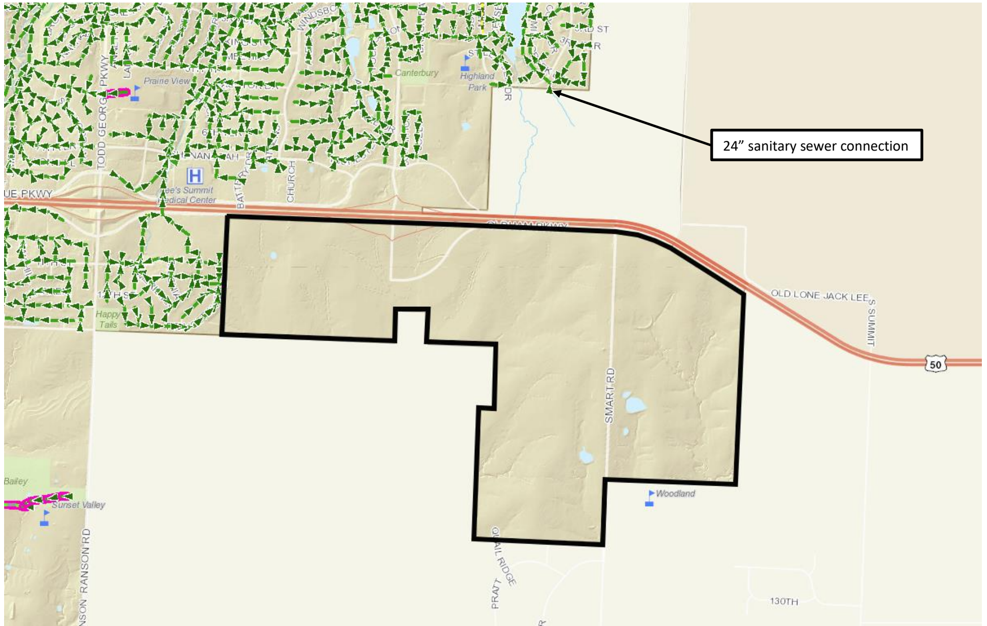
Existing Sanitary Sewer Infrastructure
