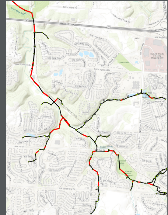
10-year Design Storm
