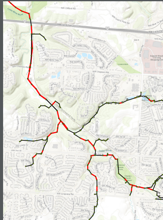
50-year Design Storm
