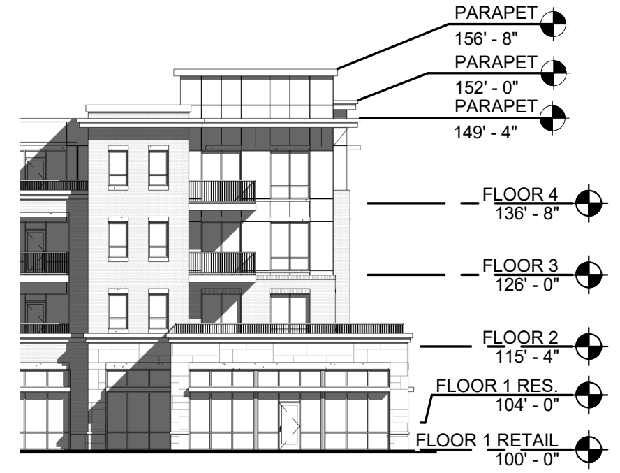
Partial South Elevation
