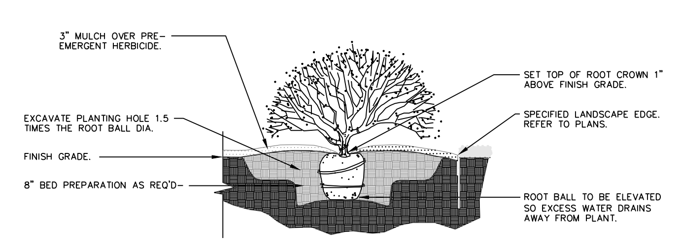
4 SHRUB PLANTING NTS
