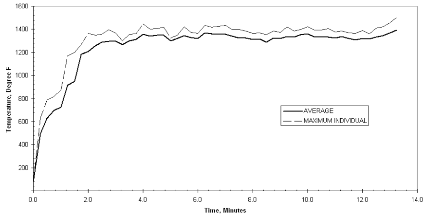
Figure 23 - Plot of Temperatures of Bottom of Wood Trusses vs. Time for Assembly No. 2
