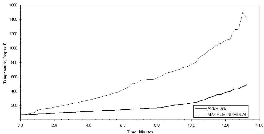
Figure 43 – Plot of Temperature of the Carpet Padding vs. Time
