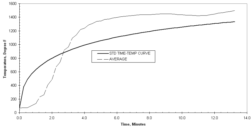
Figure 33 – UL263 (ASTM E119) Standard Time Temperature Curve and Average Furnace Temperature vs. Time for Assembly No. 3
