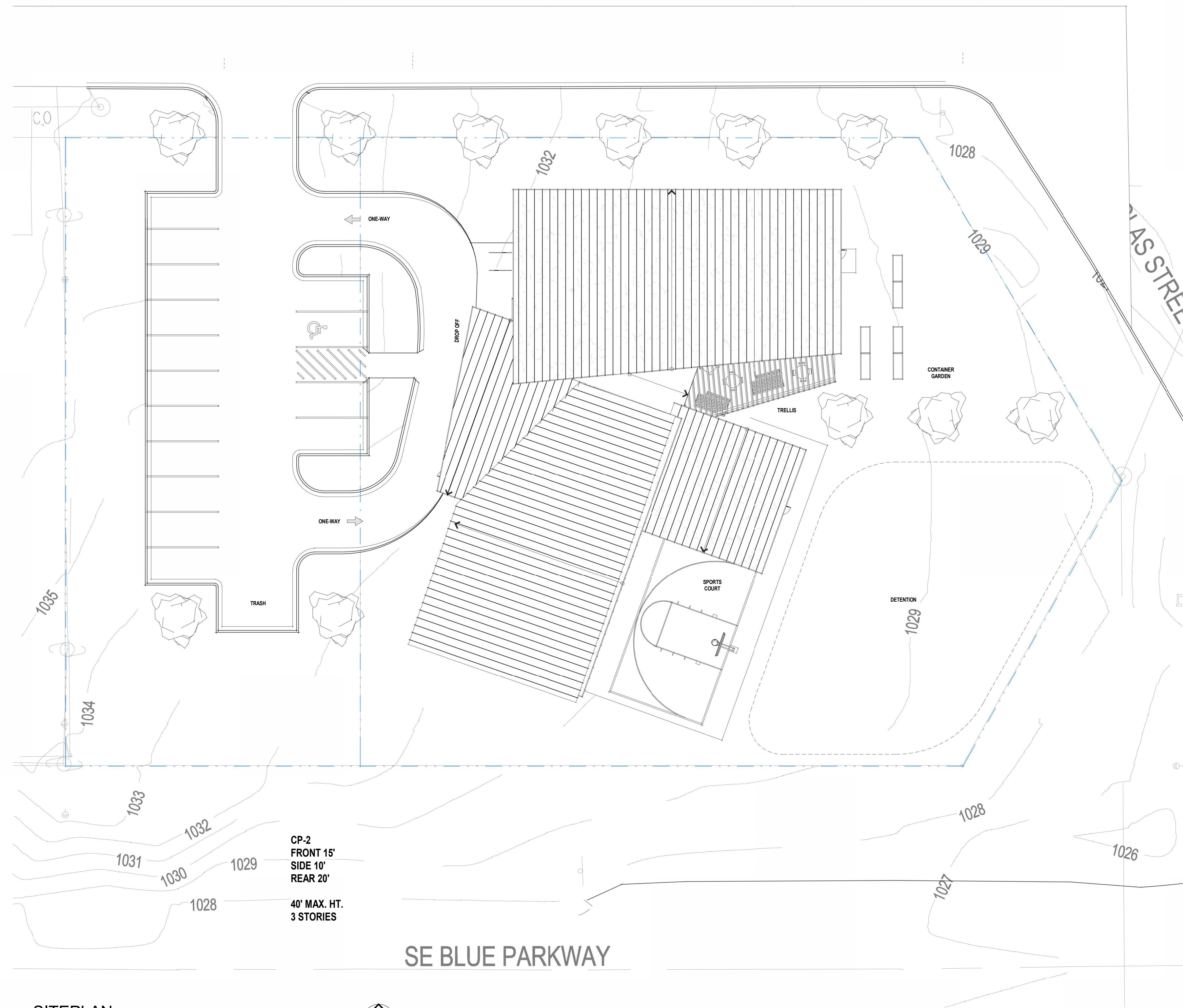
1 SITEPLAN 1/16" = 1'-0"
