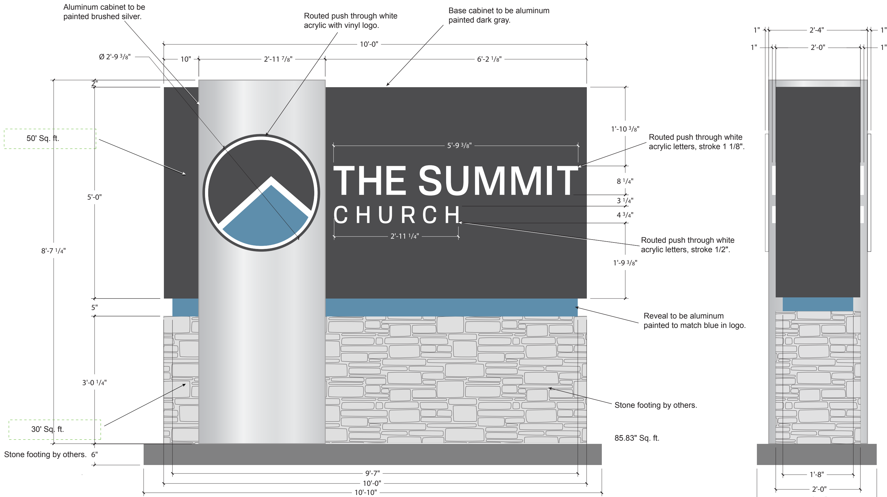
A Front view scale: 3/4" = 1'-0"
