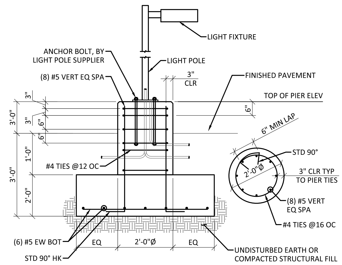
TYPICAL LIGHT POLE BASE DETAIL SCALE: NONE
