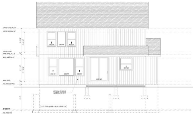
1 REAR ELEVATION 1/4" = 1'-0" WHEN PRINTED ON 24"x36" / ARCH D PAPER SIZE
