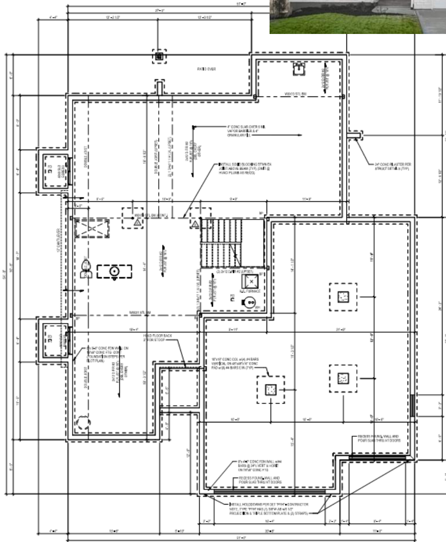
1 FOUNDATION PLAN 1/4" = 1/4"
