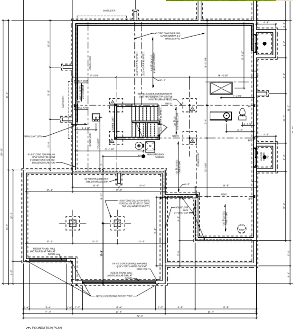
1 FOUNDATION PLAN 1/4" = 1'-0"
