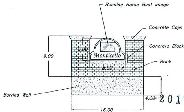
DESIGN, GRAPHIC, OR DRAWING OF THE PROPOSED SIGN WITH DIMENSIONS
