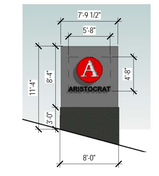
Monument Sign 1/8" = 1'-0"
