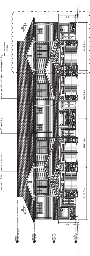
1 4 plex elevation - front Scale: 1/8"=1'-0"
